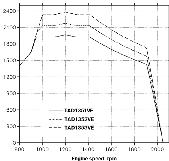
Torque, Nm
