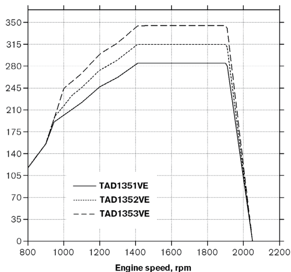
Torque, Nm
